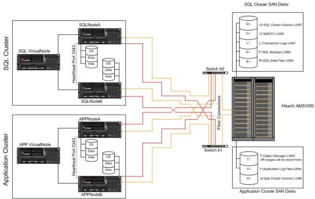
ImageNow Clustered Environment
