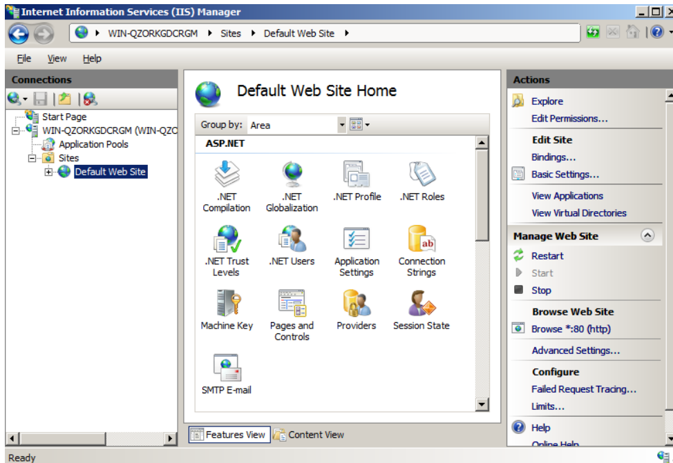
Figure 5-13: IIS Manager
